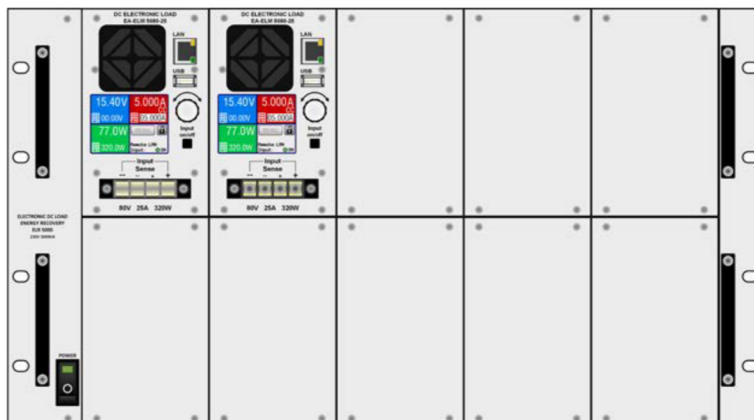
Front view of a partly equipped rack
