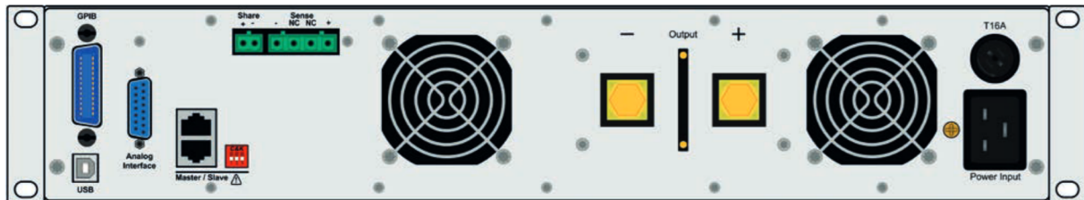
Rear view with option 3W
