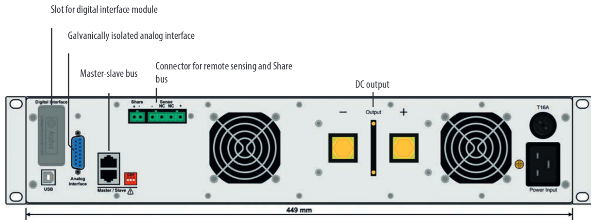
Rear view of base model
