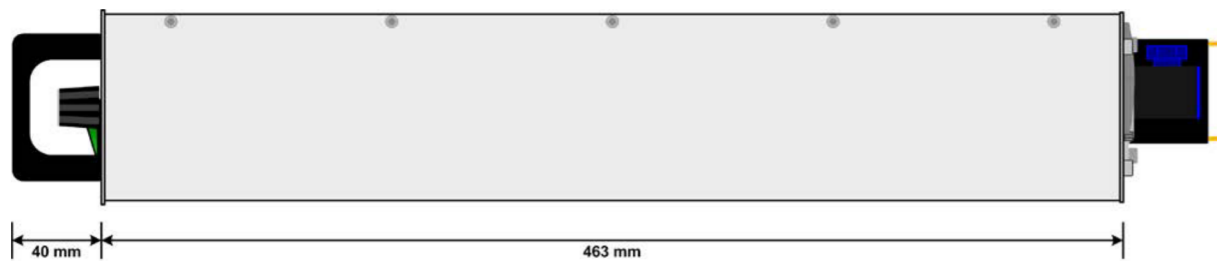
Side view of base model
